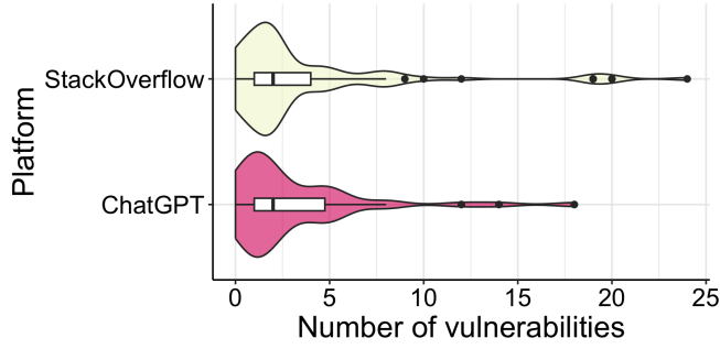
Figure 2. Number of vulnerabilities in the code snippets in each platform.
